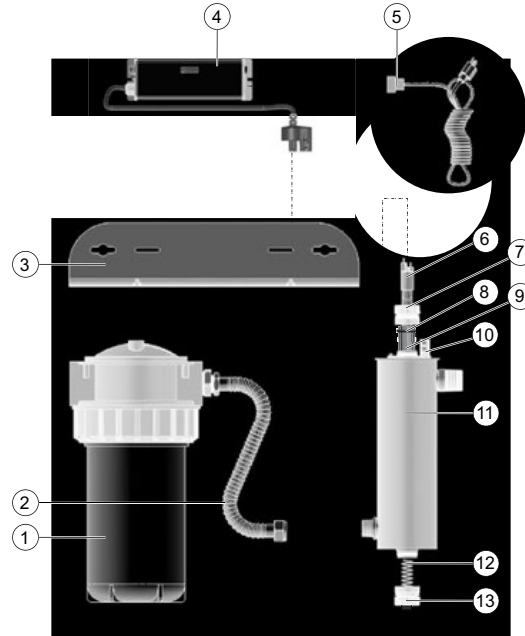
Figure 1 System Components
