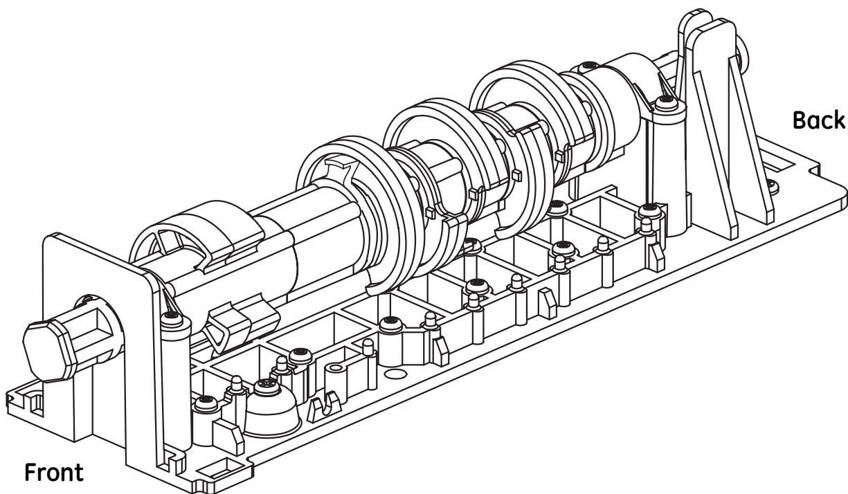
Figure 25 Cam Assembly
