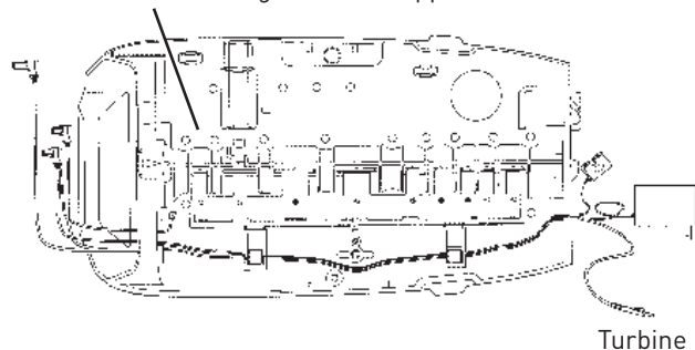
Figure 18 - Wire Harness Routing
