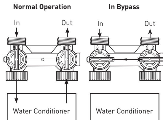
Figure 5 Series 256 bypass for use with 255 valve body
