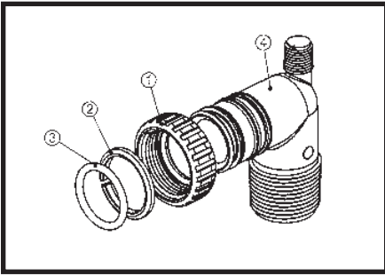
101639 - Fitting 1" PVC Male NPT
