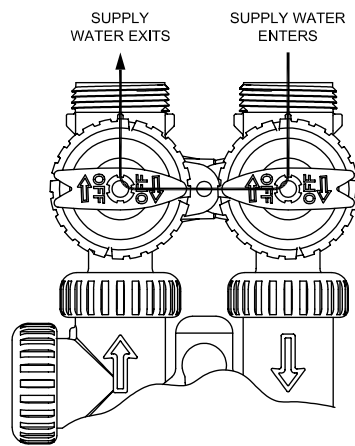
BYPASS OPERATION
