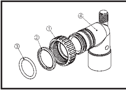
101640 - Fitting 3/4" & 1" PVC Solv 90
