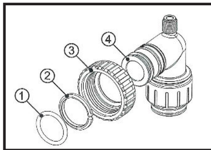
108478 - Fitting 3/4" John Guest QC
