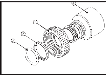
101648 - Fitting 1-1/4" & 1-1/2" Brass Sweat
