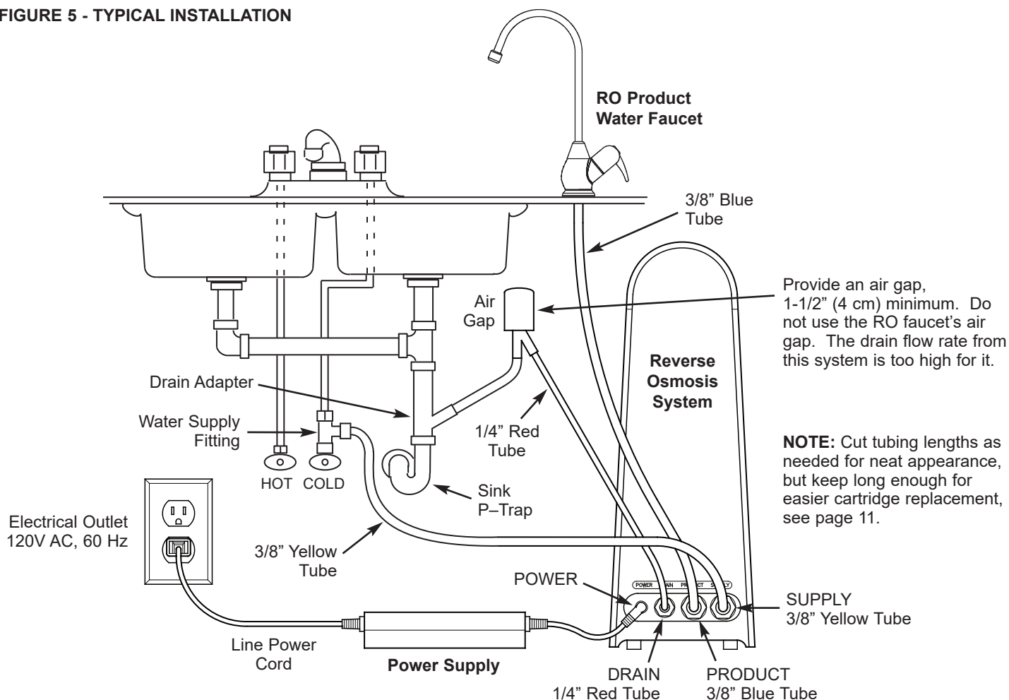
FIGURE 5 - TYPICAL INSTALLATION
