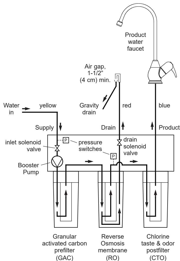
FIGURE 7 - SYSTEM DIAGRAM
