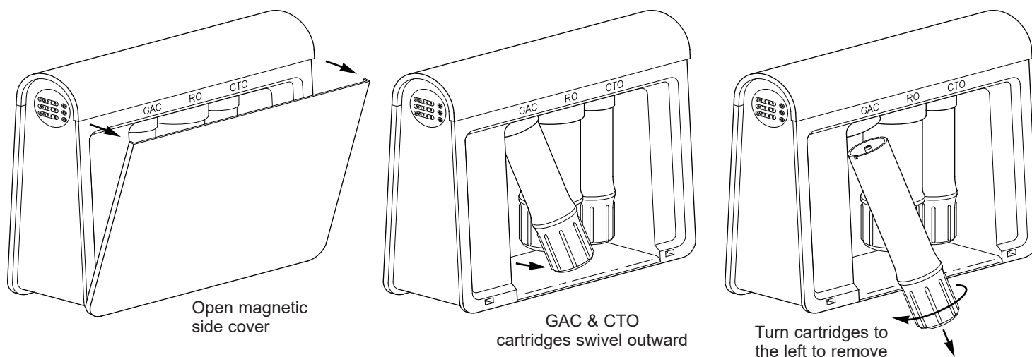
FIGURE 9 - REPLACE FILTER CARTRIDGES
