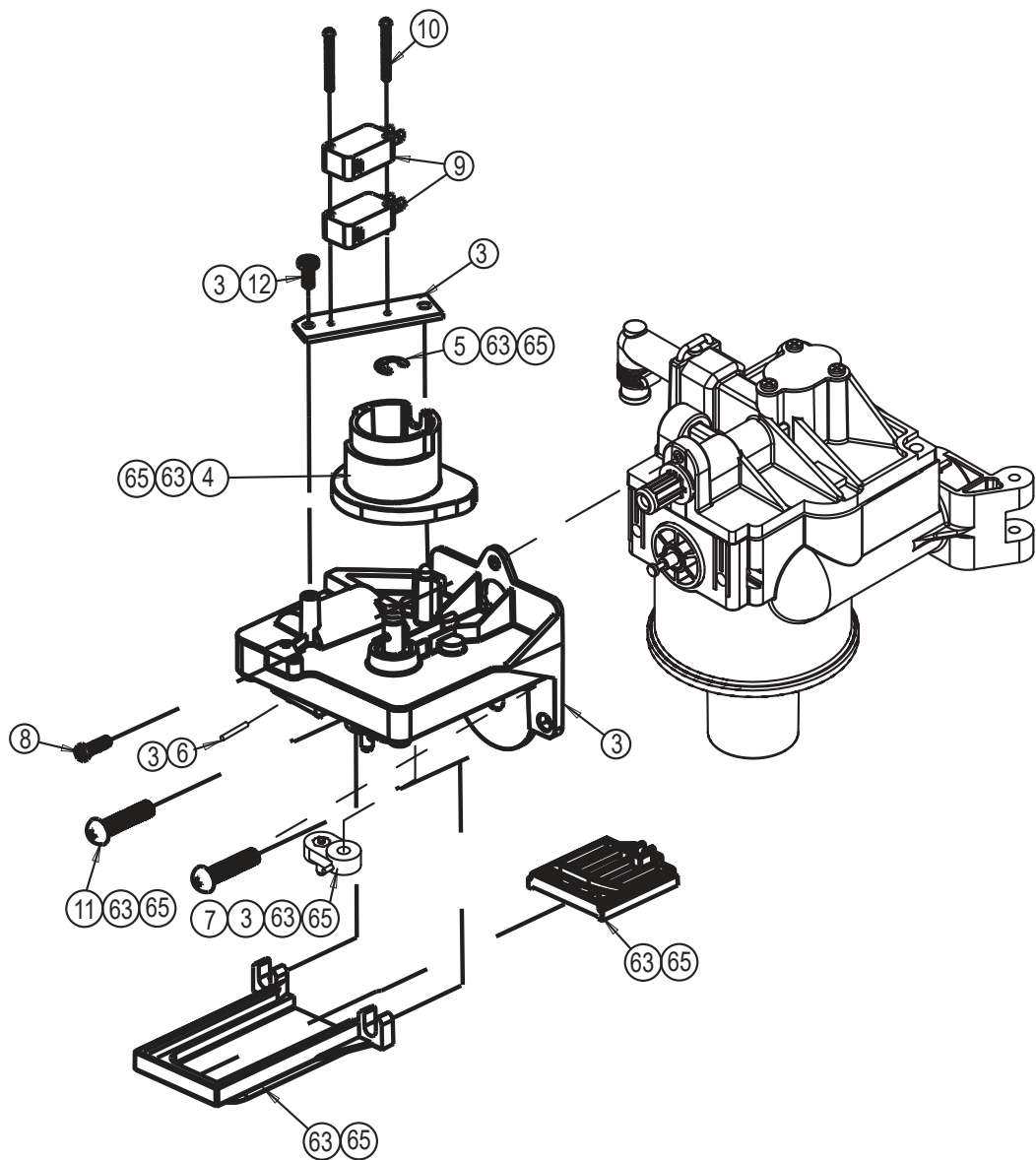
Figure 4. 1” Softener Valve
