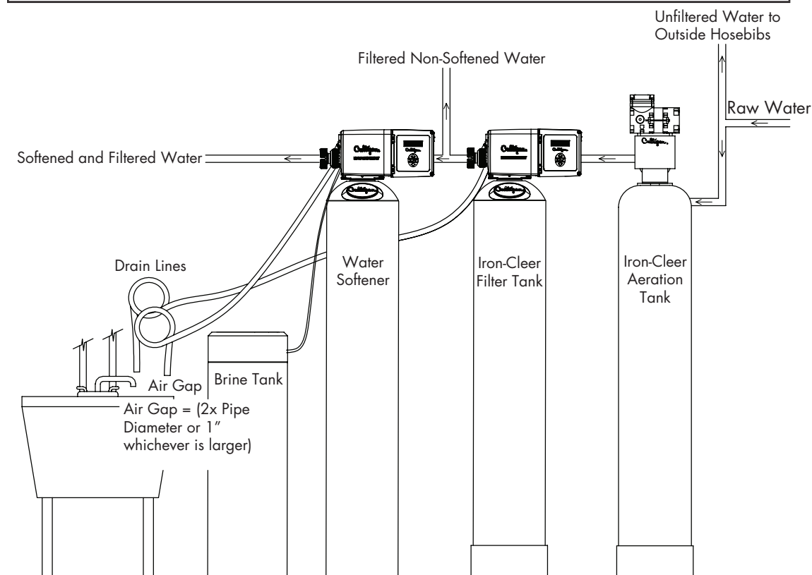
Figure 3. Iron-Clear system filter placement.
