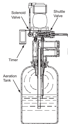
Figure 2. Air Recharge Cycle.
