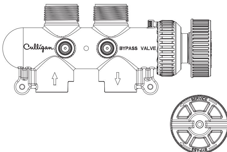
Figure 4. Bypass valve.
