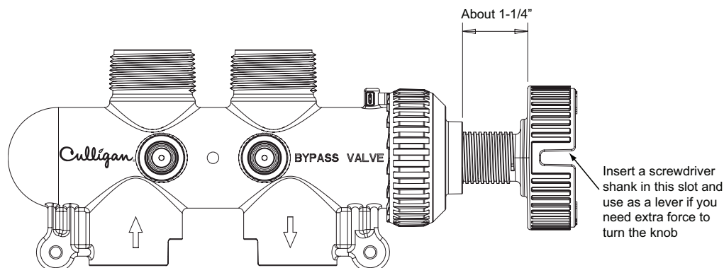
Figure 5. Service valve.
