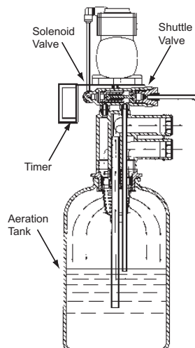
Figure 1. Aeration Service Cycle.
