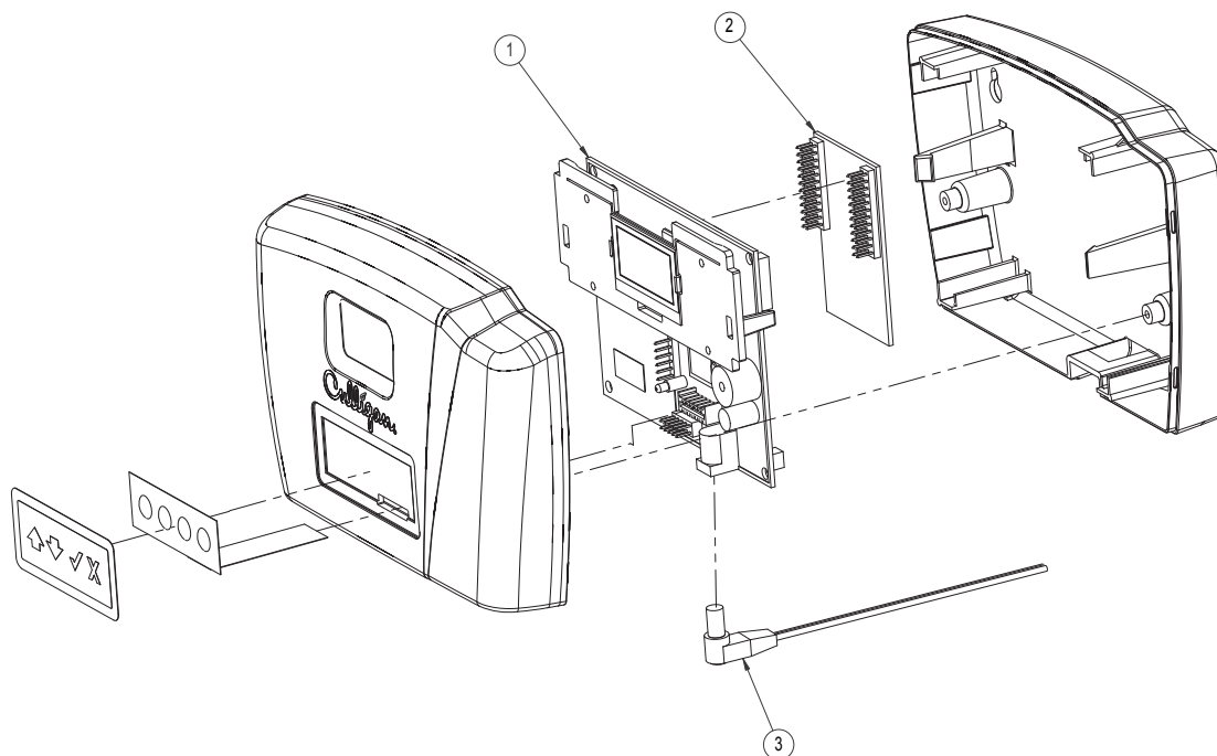
Figure 3. Remote display
