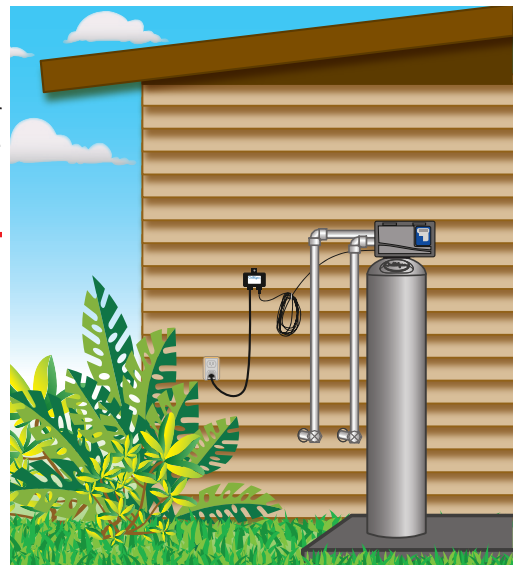
Figure 5. Outdoor installation
