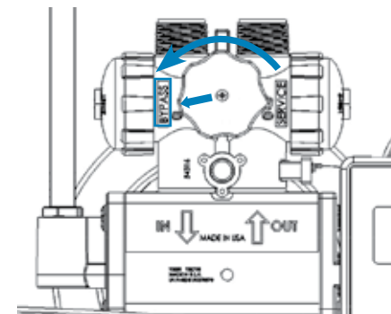
Bypass Position
