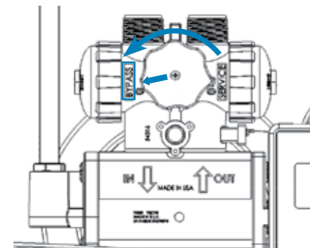
Bypass Position
